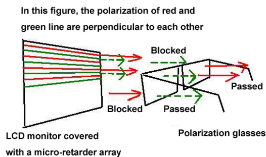
Figure 14: This figure shows how the LCD monitor present stereo with polarization glasses. The light coming from its adjacent rows has perpendicular polarization direction
