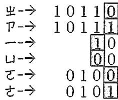
Figure 5 The example of bit mask technology
