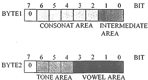
Figure 4 The two byte structure of Chinese character pronunciation
