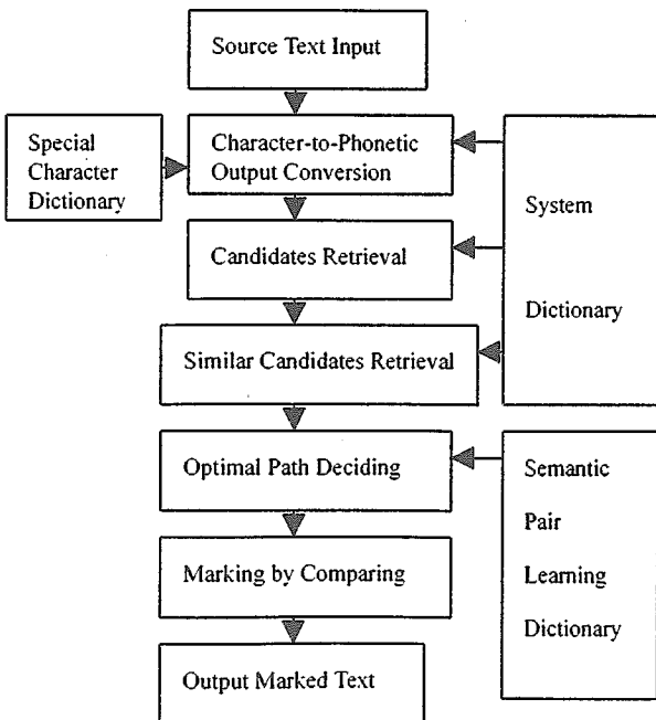
Figure 6 The processing flow of the proposed Chinese revision system
