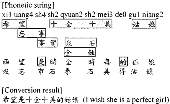
Figure 3 The example of phonetic-input-to-character conversion for Chinese
